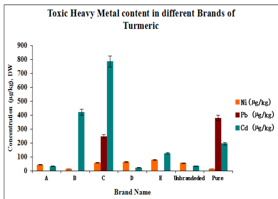
Figure 6: Ni Pb and Cd content in turmeric by GF AAS
