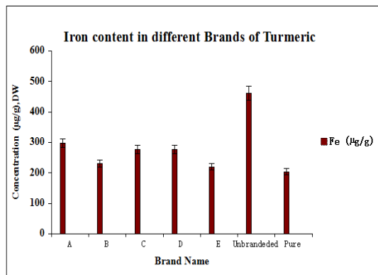
Figure 3: Fe content in turmeric by flame AAS
